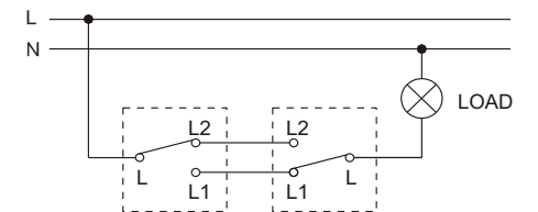
Terminal drawing
