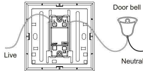
Terminal drawing
