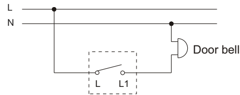
Terminal drawing
