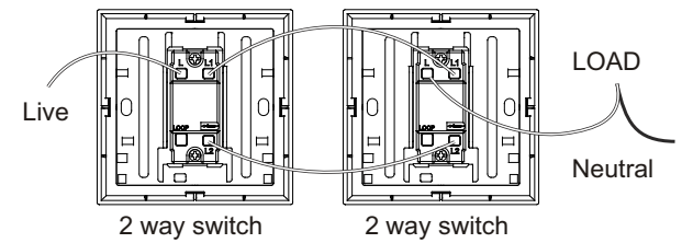
Terminal drawing
