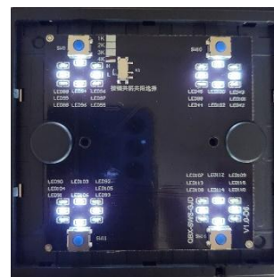
White, Yellow LED locations (behind faceplate)
