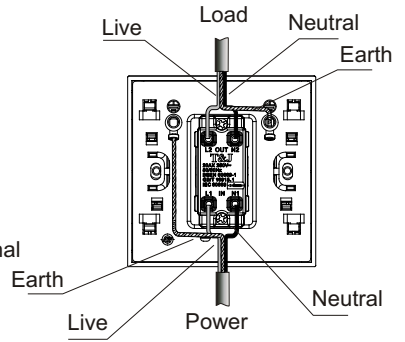
Wiring diagram 1
