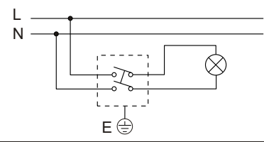
Wiring diagram 2
